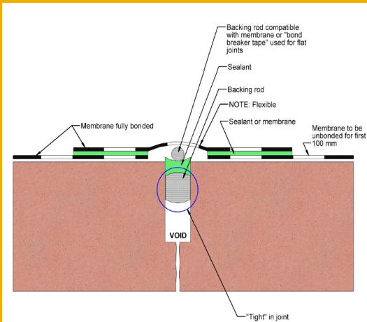
PEDESTRIAN TRAFFIC FLOOR JOINTS (Sealant is Floor Level)
